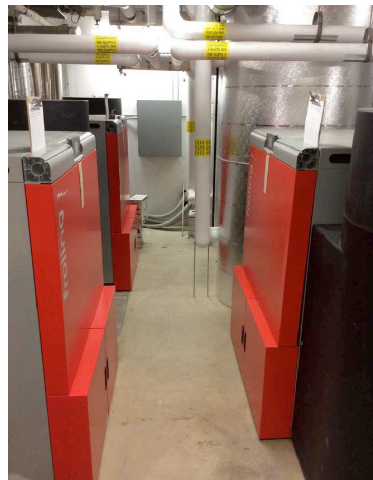
Three Fröling P4 80/100 pellet boilers
