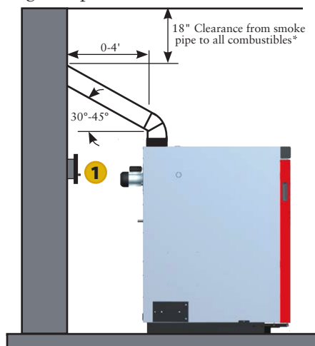
Boiler connected to chimney with connecting flue at 30-45° to help prevent ash build-up in flue.
