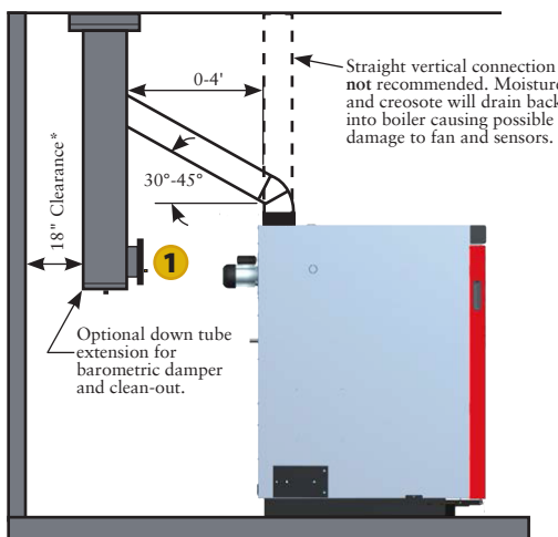
Boiler connected to manufactured chimney.
