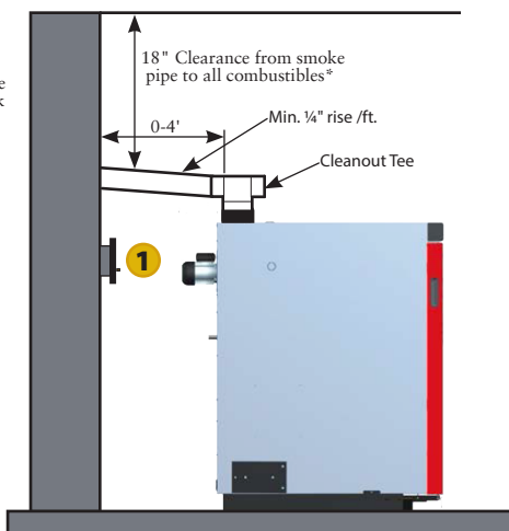
Boiler connected to chimney with minimum ¼" rise per foot. A cleanout tee is recommended for easy ash cleanout.
