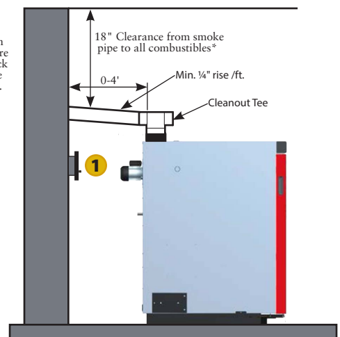
Boiler connected to chimney with minimum ¼" rise per foot. A cleanout tee is recommended for easy ash cleanout.
